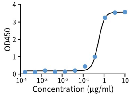
Figure 1. Immobilized 2019-nCoV Spike Protein RBD (新型冠状病毒S蛋白RBD区域) (P2331) at 100ng/well can bind SARS-COV-2 Spike Protein (RBD) Human Monoclonal Antibody (Clone B3), and the EC50 is less than 0.54µg/ml.
